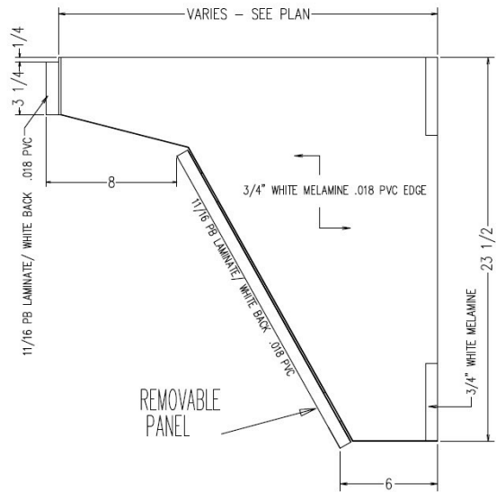
TYPICAL ADASINK
