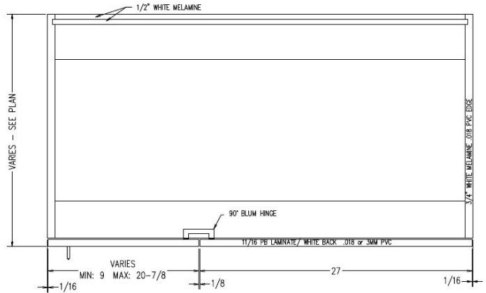
TYPICAL B1D-BLINDR TYPICAL B1D-BLINDL (OPPOSITE HAND)
