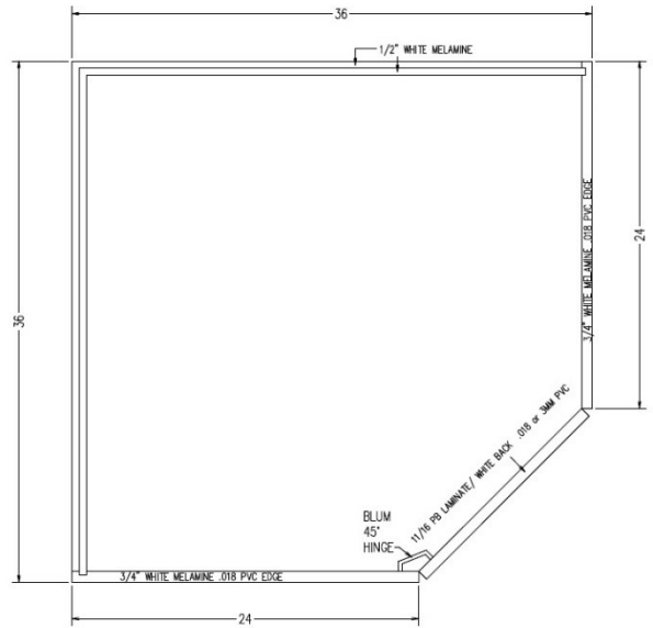
TYPICAL B1D-CORNER
