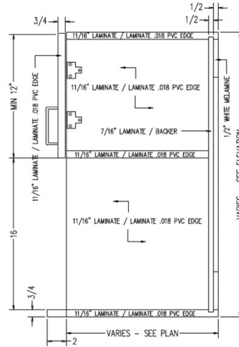
TYPICAL WMICRO (NOTE: NO LIGHT RAIL FOR THIS CABINET) SCALE: 1-1/2" = 1'-0"
